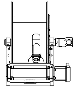
BOTTOM -XX32 4-WAY ROLLERS FRONT VIEW
