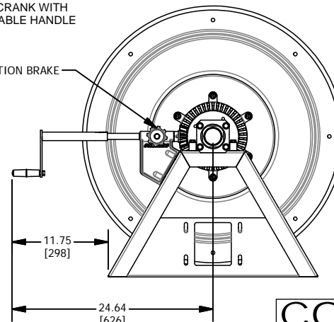
TOP -XX28 4-WAY ROLLERS FRONT VIEW
