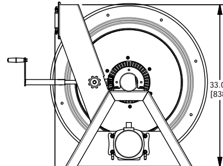
TOP -XX32 4-WAY ROLLERS SIDE VIEW
