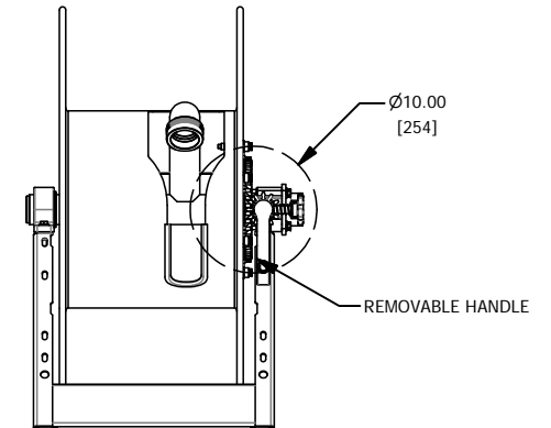
TOP -XX32 4-WAY ROLLERS FRONT VIEW
