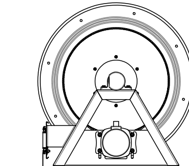
BOTTOM -XX32 4-WAY ROLLERS SIDE VIEW
