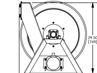
TOP -XX28 4-WAY ROLLERS SIDE VIEW
